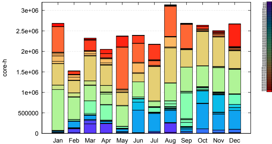
SCC statistics 2021
